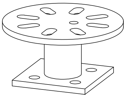
3D VIEW Scale 1:5
